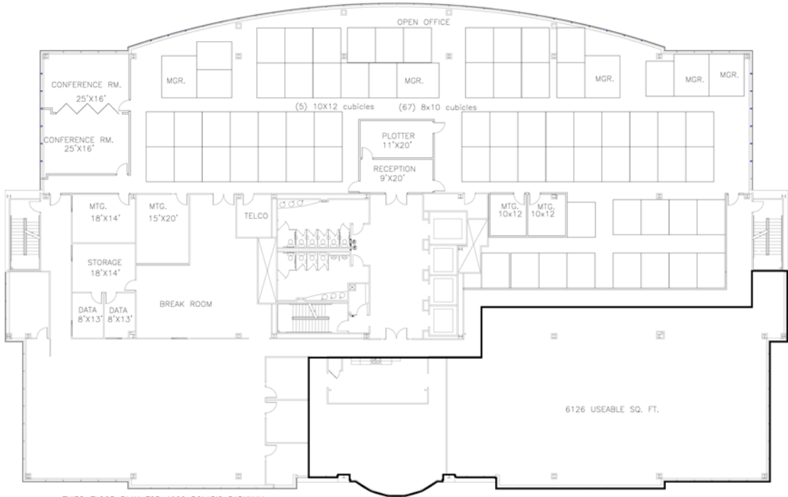
THIRD FLOOR PLAN FOR 1900 POLARIS PARKWAY
