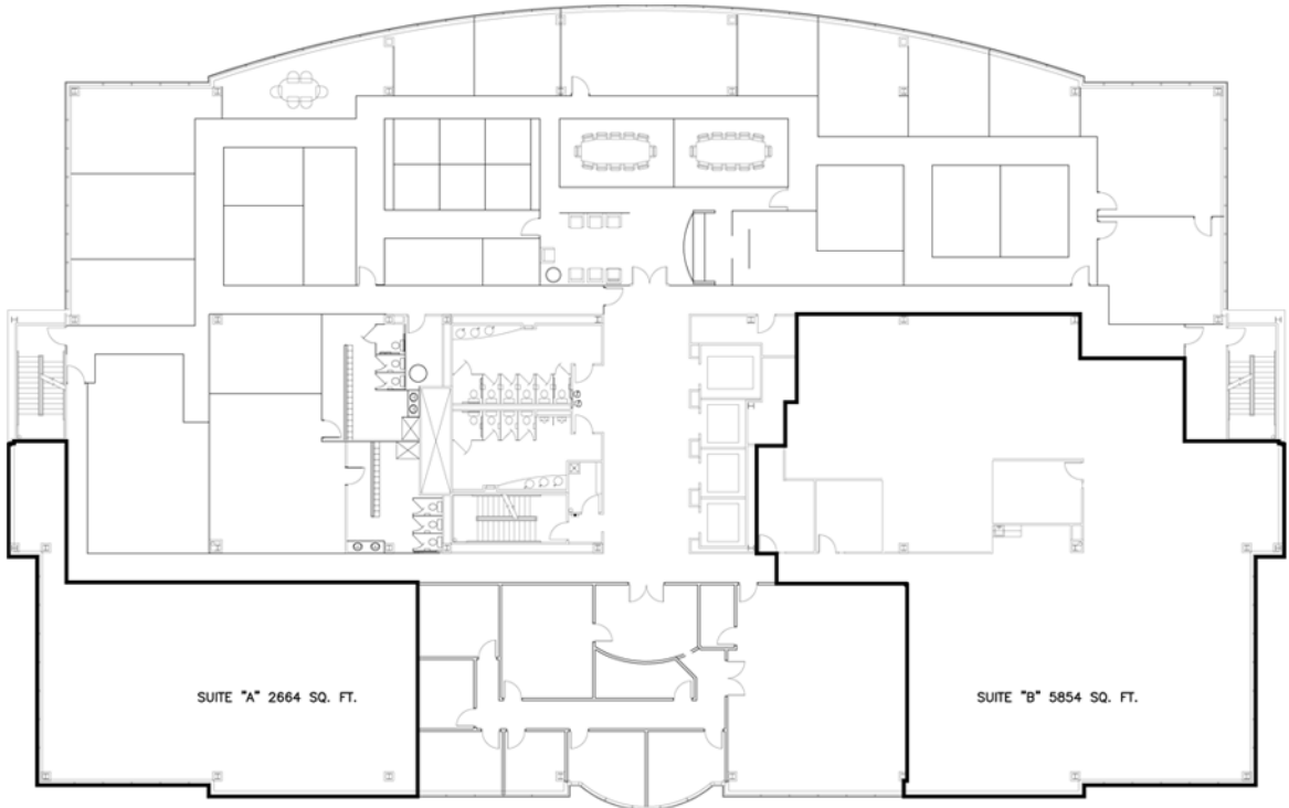
FOURTH FLOOR PLAN 1900 POLARIS PARKWAY
